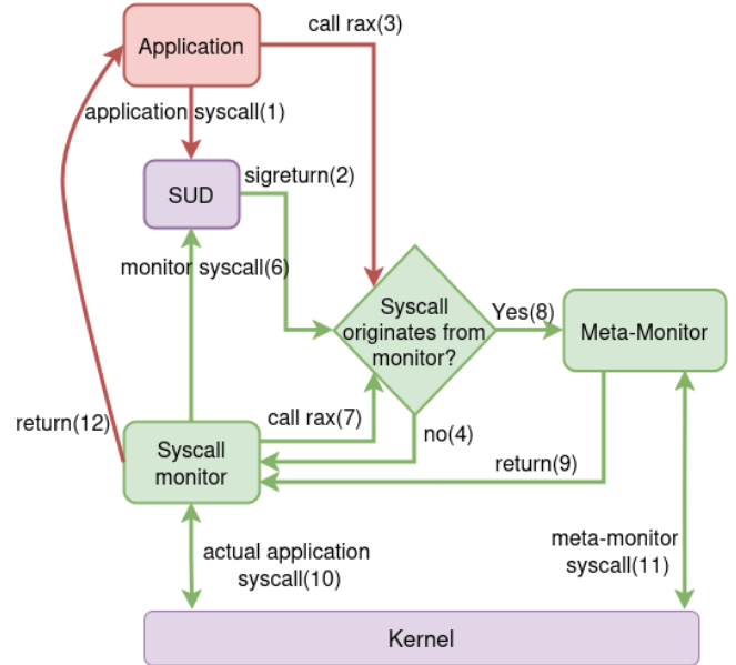
Figure 2: Secpoline system call interposition control-flow. All the trusted components are indicated in green, and transitions between trusted components are marked with a green arrow. The untrusted component is marked in red, transitions from the untrusted application to the trusted monitor and vice versa are marked in red. All kernel components are marked in purple.
